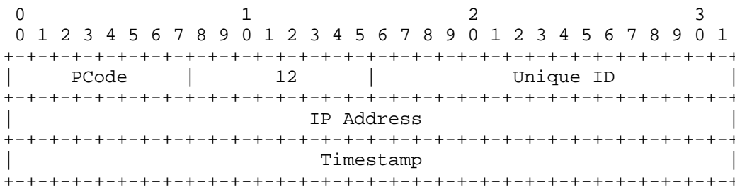
Figure 29. Name & RName
