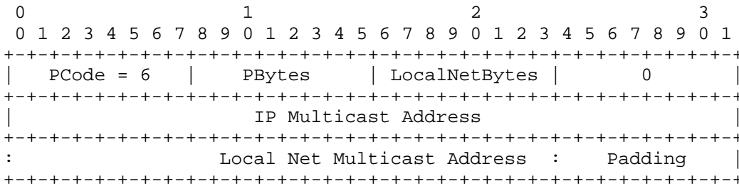
Figure 28. MulticastAddress
