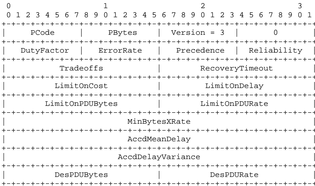
Figure 24. FlowSpec & RFlowSpec
