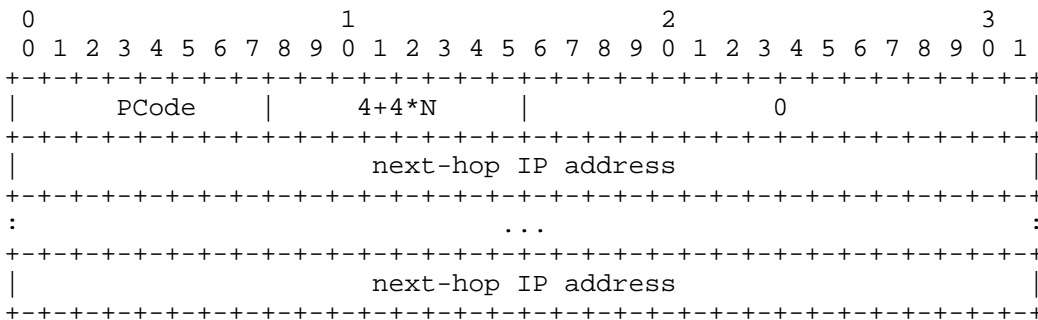
Figure 35. SrcRoute
