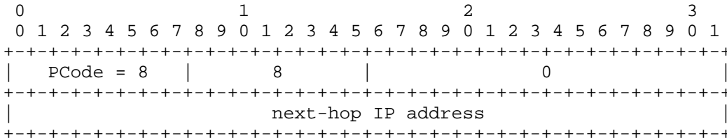
Figure 30. NextHopIPAddress
