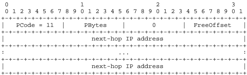
Figure 34. RecordRoute
