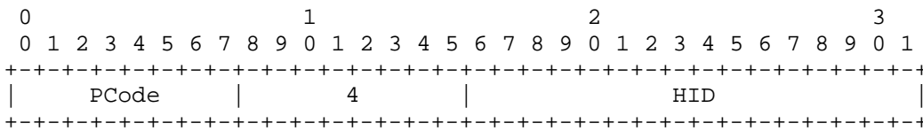
Figure 27. HID & RHID
