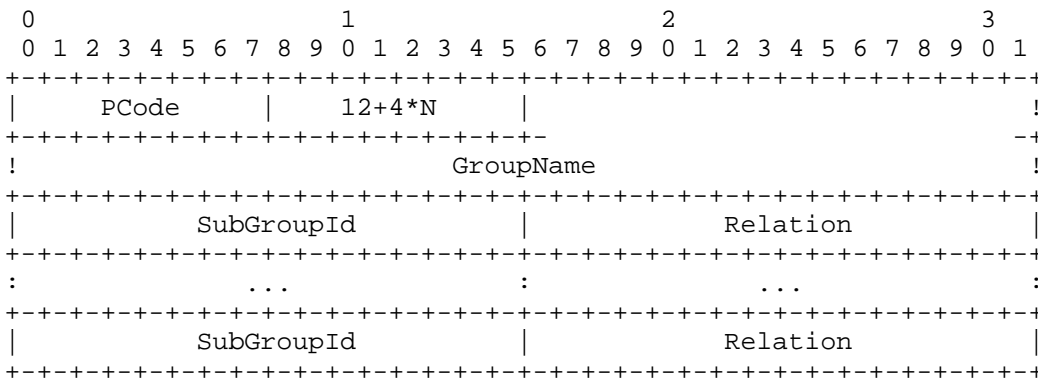
Figure 26. Group & RGroup
