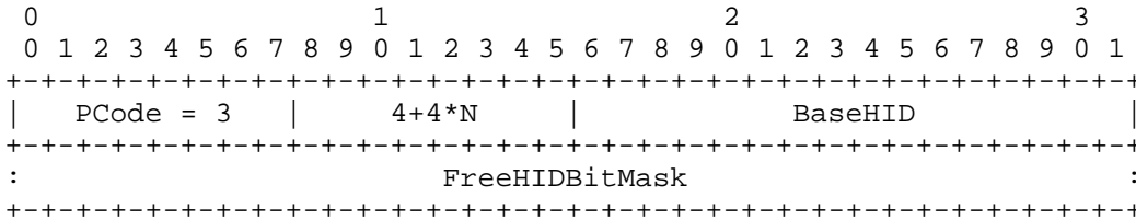
Figure 25. FreeHIDs
