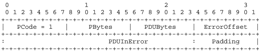
Figure 23. ErroredPDU
