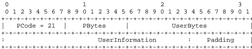
Figure 38. UserData
