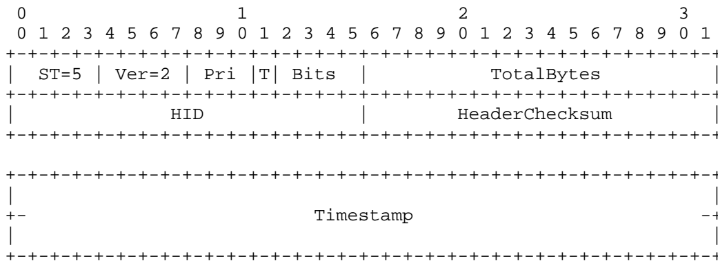
Figure 21. ST Header
